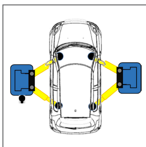
2-Stage arms for 4 Ton Floor Plate
